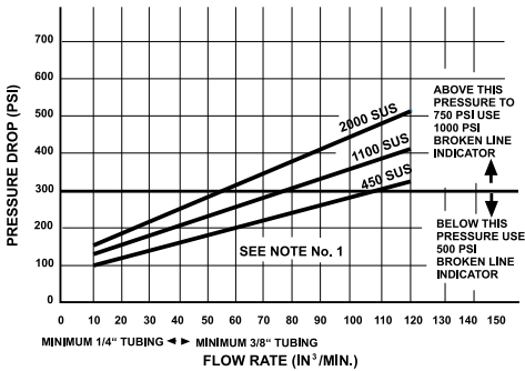
Typical Operating Pressure For 2 Stage “MX” to “MSP” System
