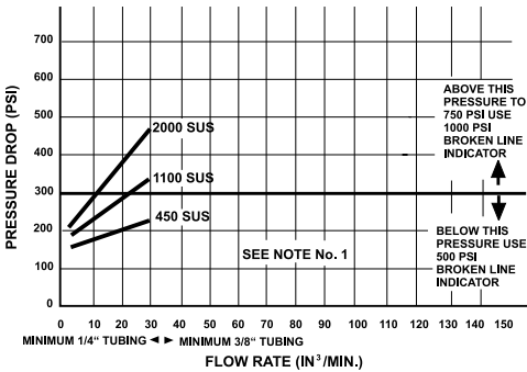
Typical Operating Pressure For 2 Stage “MSP” Systems
