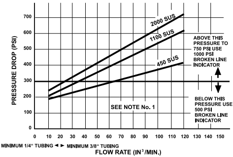
Typical Operating Pressure For 2 Stage “MX” to “MSP” System
